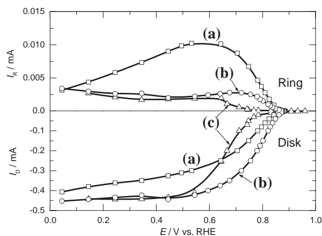
Figure 1. Rotating ring-disk electrode voltammograms for oxygen reduction on (a) HT-Co[Fe]PB/C, (b) HT-Cu[Fe]PB/C, and (c) bright Pt in 1 M potassium phosphate buffer solution (pH 7.6) saturated with oxygen. The collection efficiency of the ring-disk electrode is 0.48. The rotation rate of the electrode was 1500 rpm. The ring electrode potential was set at 1.35 V vs. RHE.
