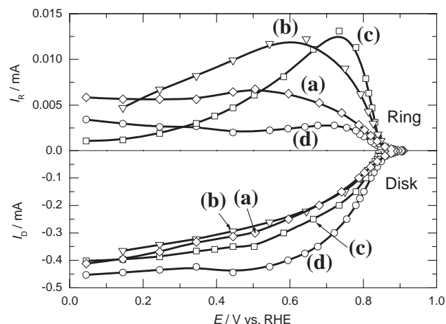
Figure 2. Rotating ring-disk electrode voltammograms for oxygen reduction on (a) HT-Fe[Fe]PB/C, (b) HT-Co[Co]PB/C, (c) HT-Cu[Co]PB/C, and (d) HT-Cu[Fe]PB/C. Other conditions were the same as in Figure 1.
