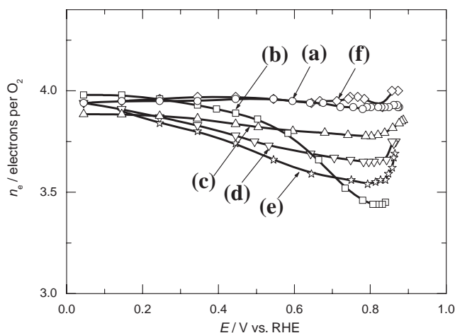
Figure 3. Average number ( n_e ) of electrons transferred per O_2 during oxygen reduction on the disk: (a) HT-Cu[Fe]PB/C, (b) HT-Cu[Co]PB/C, (c) HT-Fe[Fe]PB/C, (d) HT-Co[Fe]PB/C, (e) HT-Co[Co]PB/C, and (f) bright Pt.
